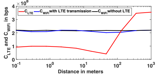
Fig. 4. Trans. rates of LTE and WiFi vs. separating distance for \kappa = 0.9
