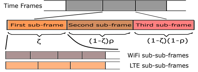
Fig. 1. Explanation of Time Division between WiFi and LTE system
