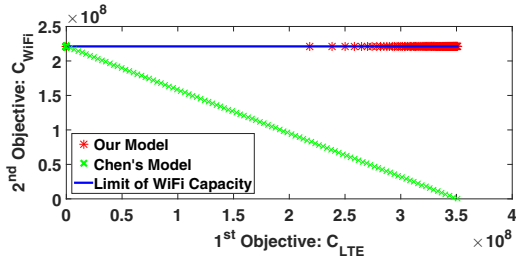
Fig. 8. Pareto curve with \kappa = 0.9 and l = 1000
