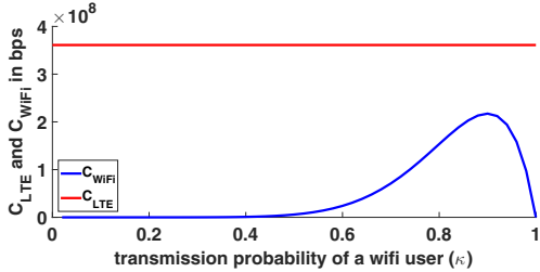
Fig. 2. Trans. rates of LTE and WiFi vs. trans. probability
